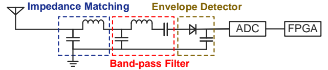
Figure 14: The circuit design of LoRa packet detector.
