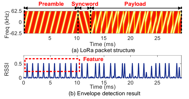
Figure 13: LoRa preamble and the corresponding RSSI profile. The ten consecutive up-chirps on LoRa preamble (top) leads to ten equally-spaced RSS pulses (below).
