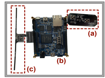
(a) LoRa packet detection (b) FPGA (c) WISP
