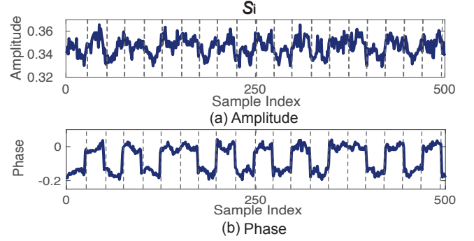
Figure 10: Reconstructed signal. (a): amplitude variation of the reconstructed signal becomes indistinguishable when carrier signal and backscatter signal are not strictly aligned. (b): the phase of this reconstructed signal shows a distinctive pattern.
