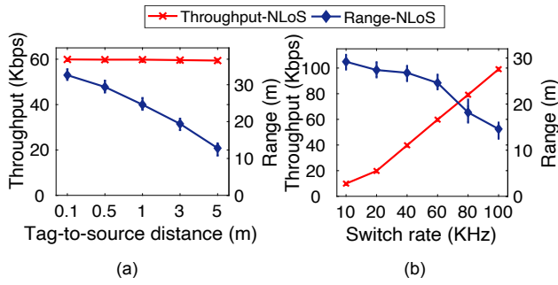
Figure 23: Aloba performance in NLoS indoor environments (penetrating one concrete wall)
