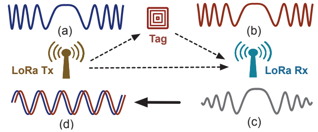
Figure 3: LoRa backscatter system. Aloba tag modulates the ambient LoRa signal using On-Off Keying. (a): carrier signal transmitted by LoRa Tx. (b): backscatter signal modulated by Aloba tag. (c): received signal is the superposition of carrier signal and backscatter signal. (d): the LoRa receiver decodes both LoRa carrier signal and backscatter signal using our demodulation algorithm.
