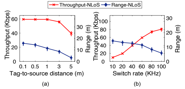
Figure 24: Aloba performance in NLoS indoor environments (penetrating two concrete walls)
