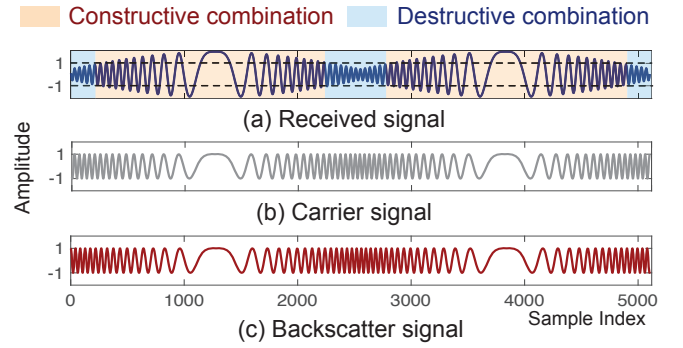
Figure 5: The received signal is the superposition of the carrier signal and backscatter signal (propagation delay of the backscatter signal is 1.8 μs). The received signal experiences periodic amplitude variation due to constructive and destructive interference.
