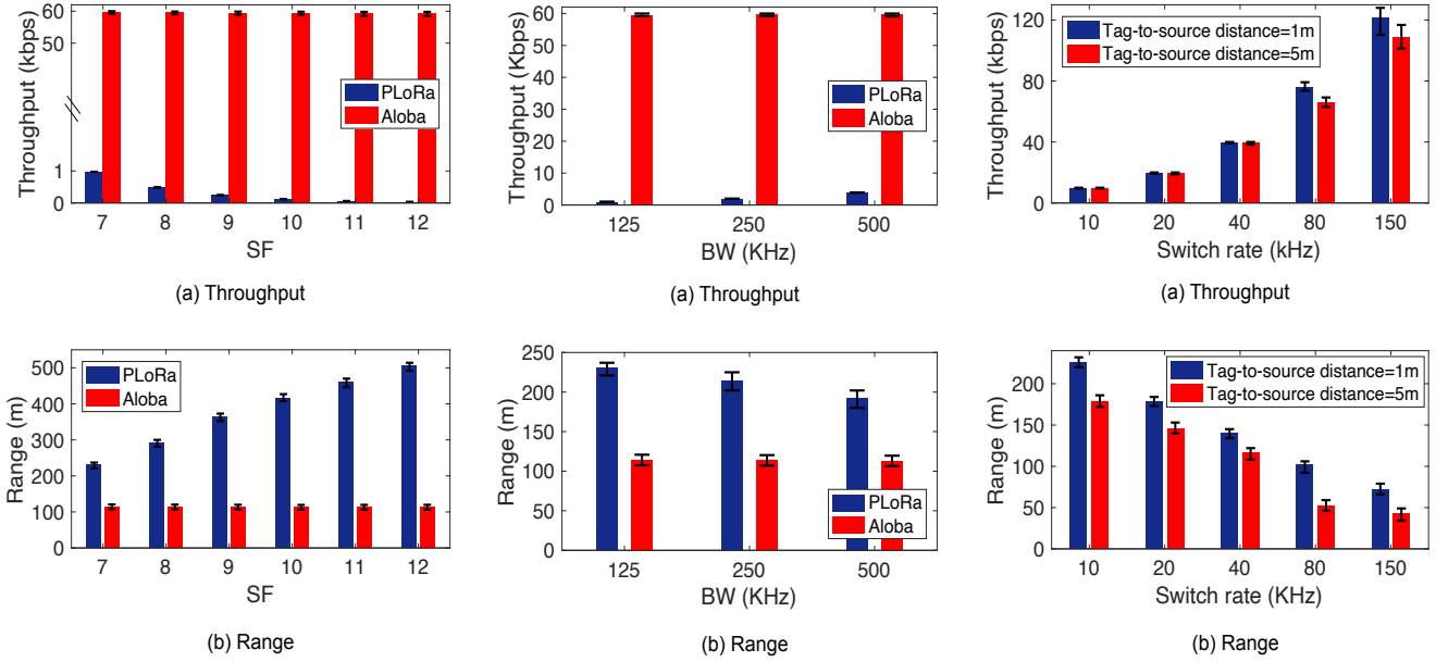
Figure 20: Performance comparison with different SF settings Figure 21: Performance comparison with different BW settings Figure 22: Performance comparison with different switch rate settings
