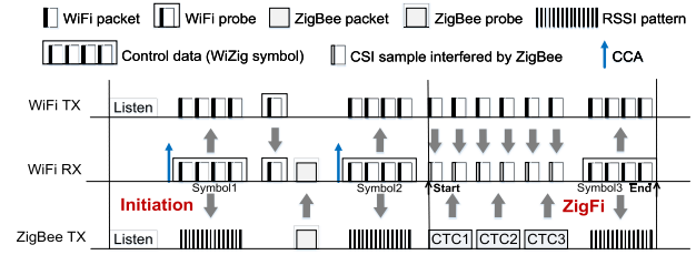
Fig. 9. The process of receiver-initiated mechanism.
