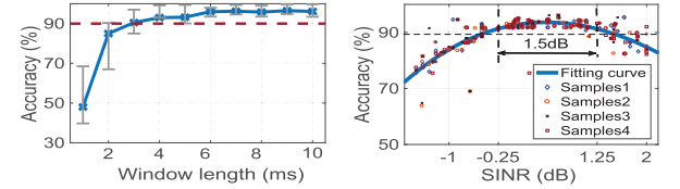
(a) The relationship between the accuracy and the window length (b) The relationship between the accuracy and the SINR
