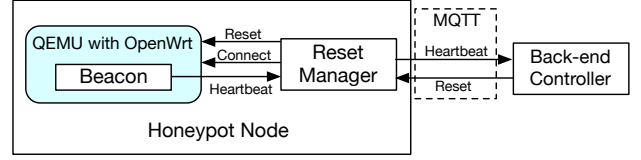
Figure 6: Heartbeat-based failure recovery.
