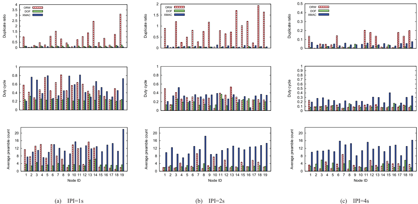
Fig. 7. Per node comparison of different system performance metrics between DOF and the other forwarding protocols in high traffic loads.
