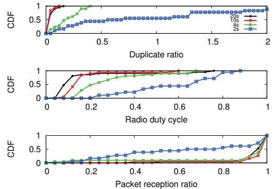
Fig. 2. The CDF of the duplicate ratio, radio duty cycle, and packet reception ratio with different traffic loads on test-bed experiment, when the sleep interval is 512ms.
