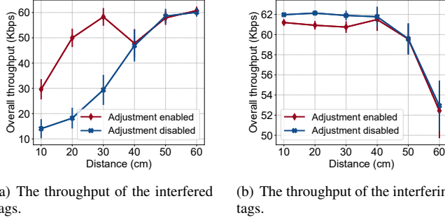
Fig. 16: Throughput comparison of tags with & w/o power adjustment in different distance settings between interfering tag and readers.
