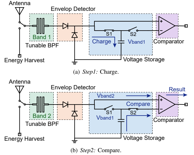
Fig. 5: The frequency band detector completes the comparison of signal strengths at two frequency bands through two steps.
