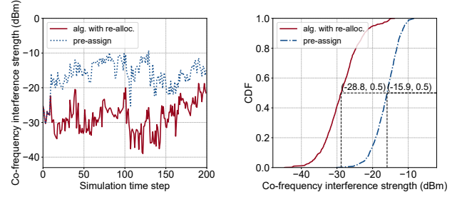
Fig. 18: Co-frequency interference strength of our algorithm and the pre-assigning method in the dynamic channel.
