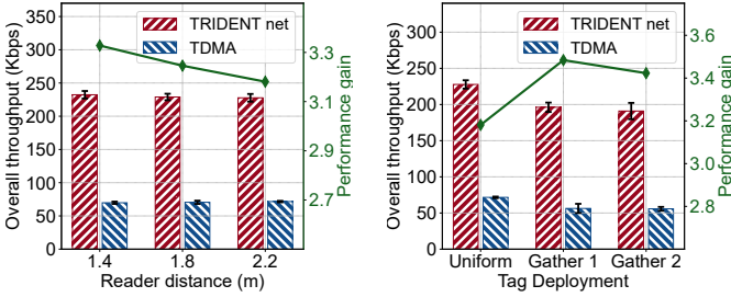
Fig. 12: Overall throughput comparison between two networks with reader density represented by the distance between readers.
