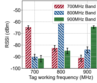
Fig. 14: The RSSI of tag signals when tags operating at various frequencies are excited by different excitation frequency bands.
