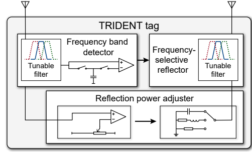
Fig. 2: The three key components of Trident tag.
