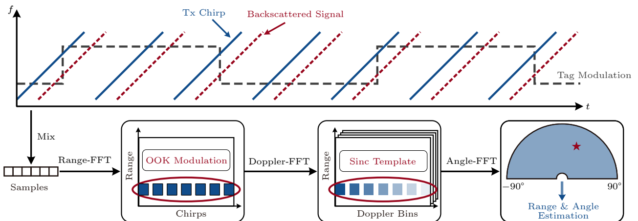
Fig.6. Concurrent tag localization and identification in Millimetro.
