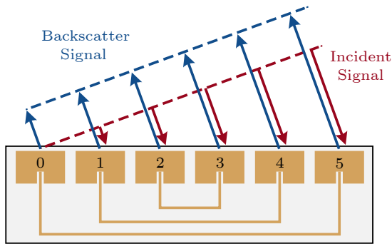
Fig.5. VAA used in mmTag [69] .
