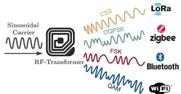
Fig.4. RF-Transformer backscatter design. CCS: Chirp Spread Spectrum, QPSK: Offset Quadrature Phase Shift Keying, QAM: Quadrature Amplitude Modulation.
