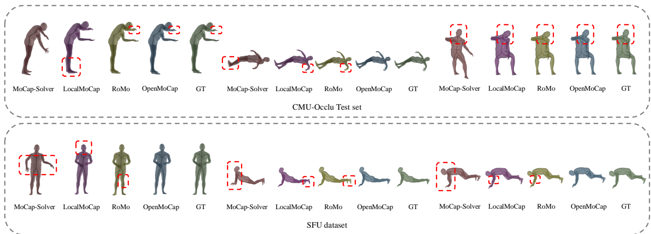
Figure 9: Qualitative evaluation of different models on CMU-Occlu test set and SFU dataset.
