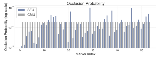
(a) Marker Occlusion Probability.
