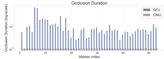
(b) Marker Occlusion Duration.
